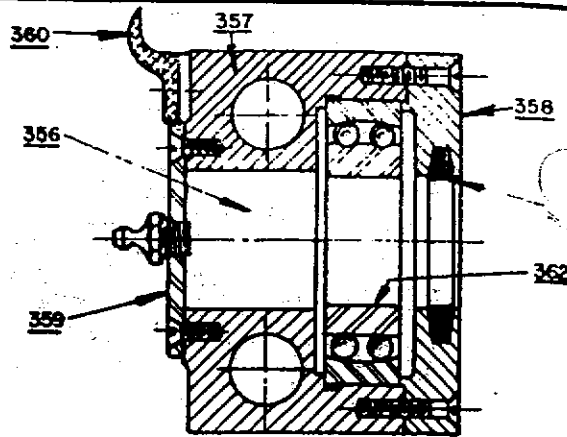
SECTION OF SPIRAL ROLL BEARINGS
