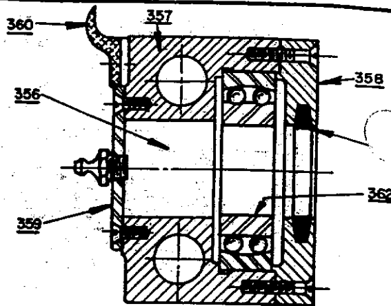
SECTION OF SPIRAL ROLL BEARINGS
